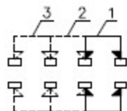
Non-shorting SCHEMATIC
