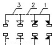
NON-SHORTING SCHEMATIC
