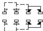
NON-SHORTING SCHEMATIC
