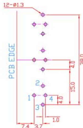
PCB LAYOUT (BOTTOM VIEW)
