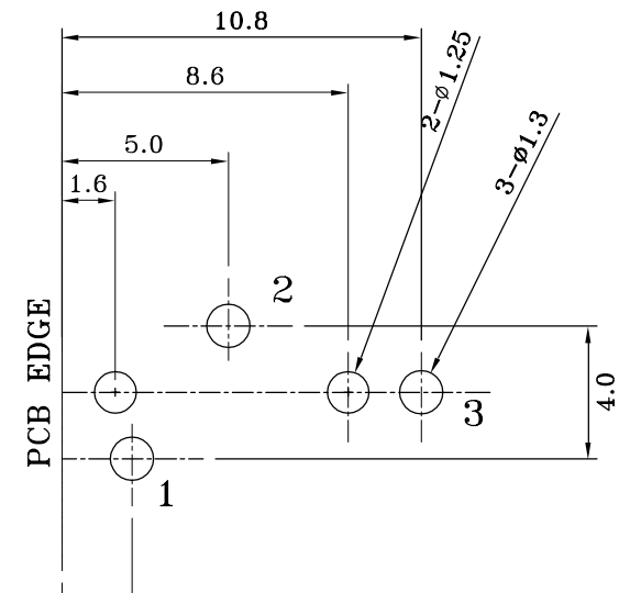
RECOMMENDED COMPONENT SIDE (PCB LAYOUT)
