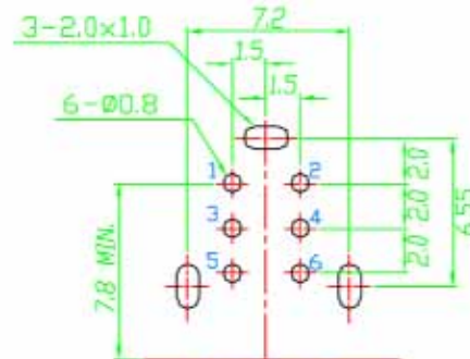
PCB EDGE COMPONENT SIDE (PCB LAYOUT)
