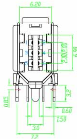
PCB EDGE COMPONENT SIDE (PCB LAYOUT)
