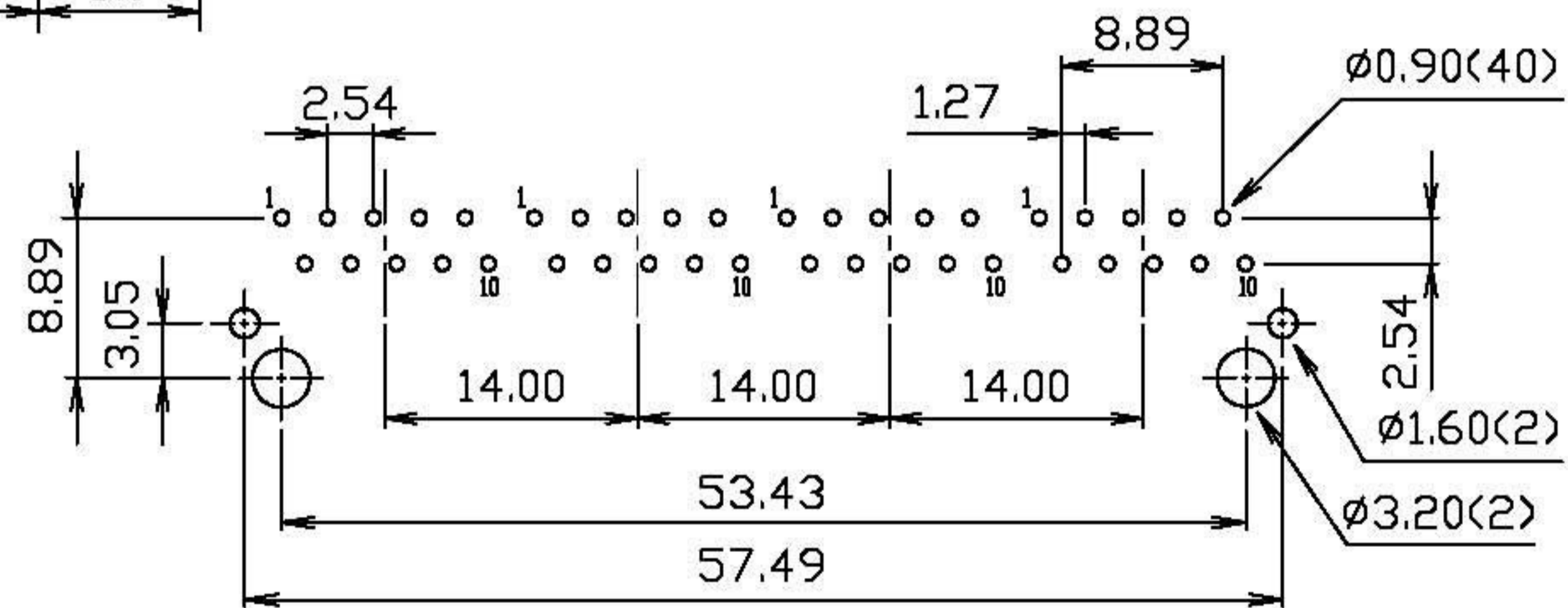
PCB LAYOUT
