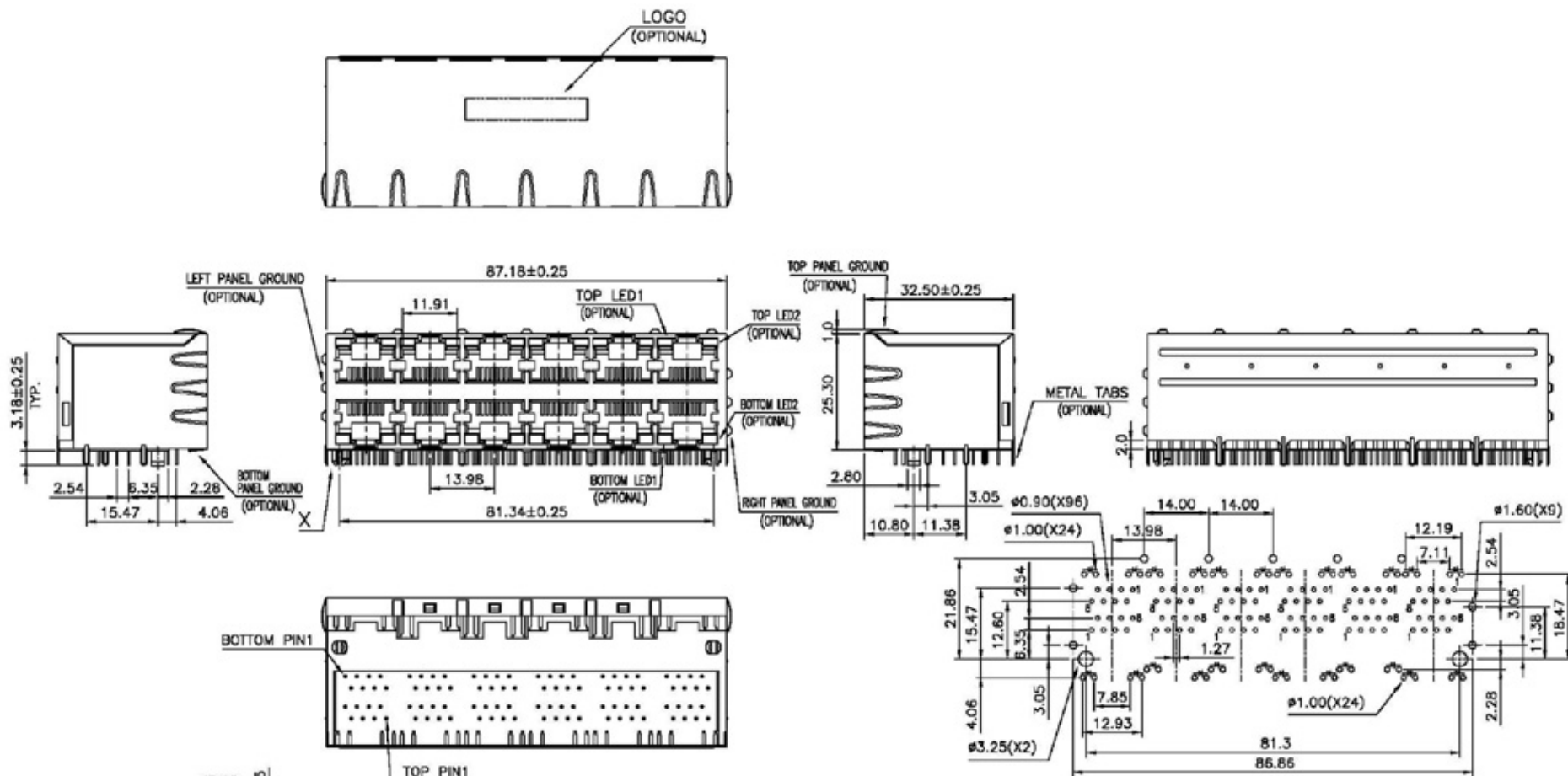
PCB LAYOUT Ref.
