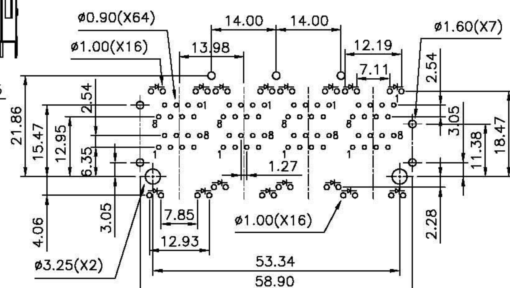
PCB LAYOUT Ref.
