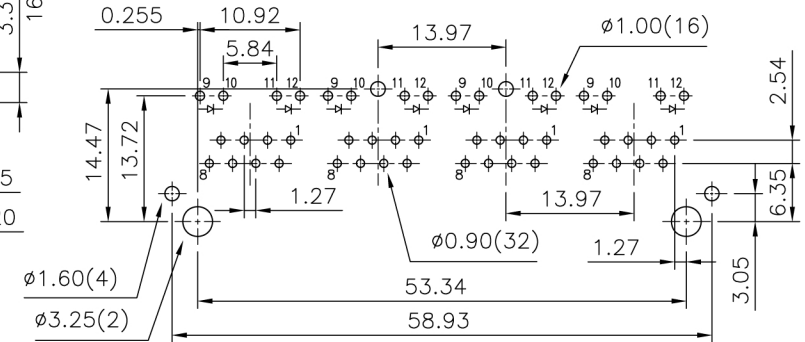
PCB LAYOUT Ref.
