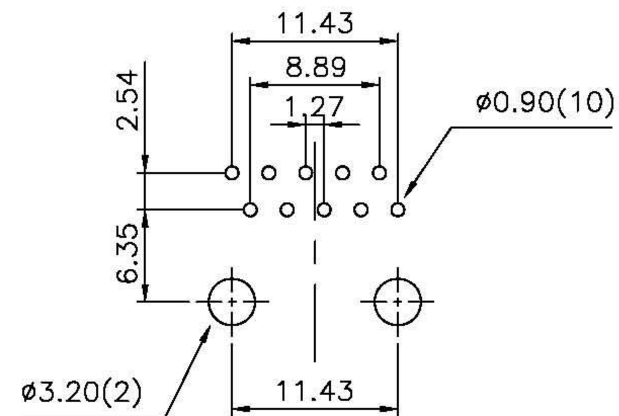
PCB LAYOUT
