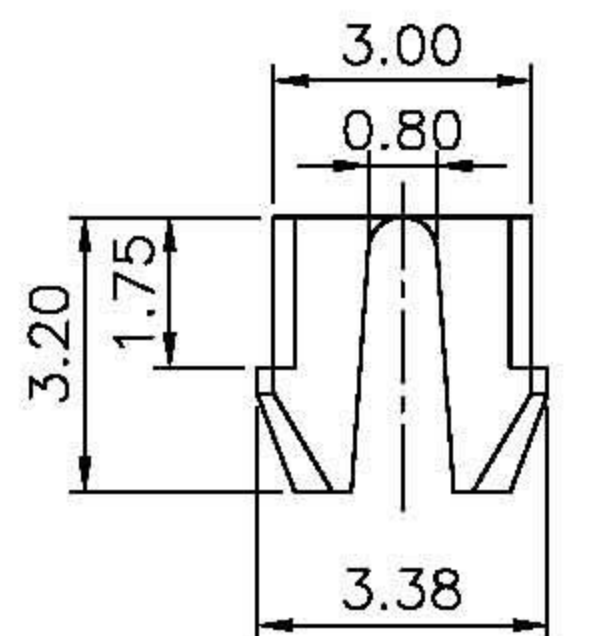
DETAIL X
