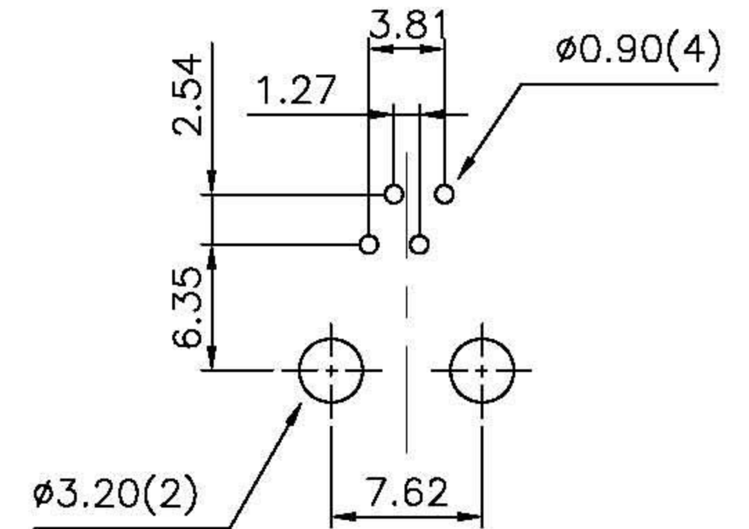
PCB LAYOUT
