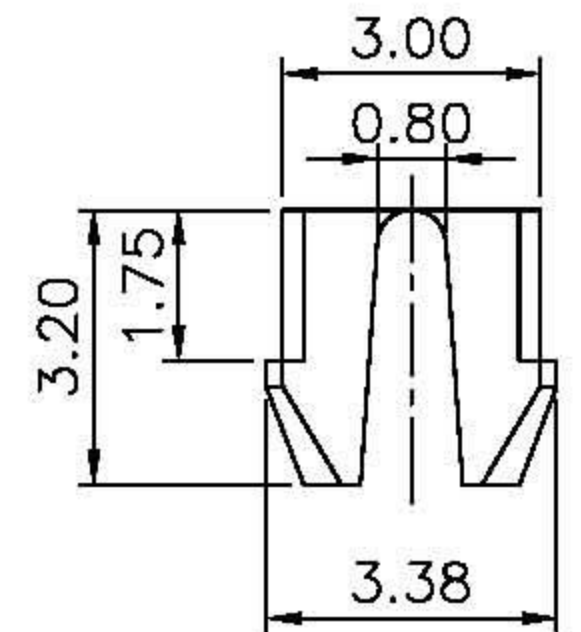
DETAIL X
