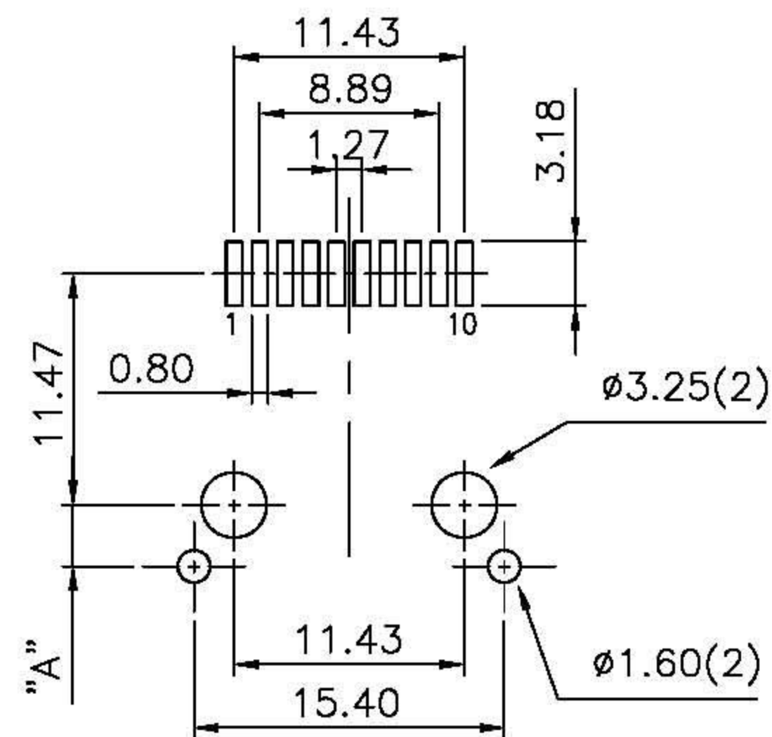
PCB LAYOUT Ref.
