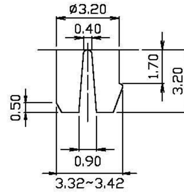
DETAIL X
