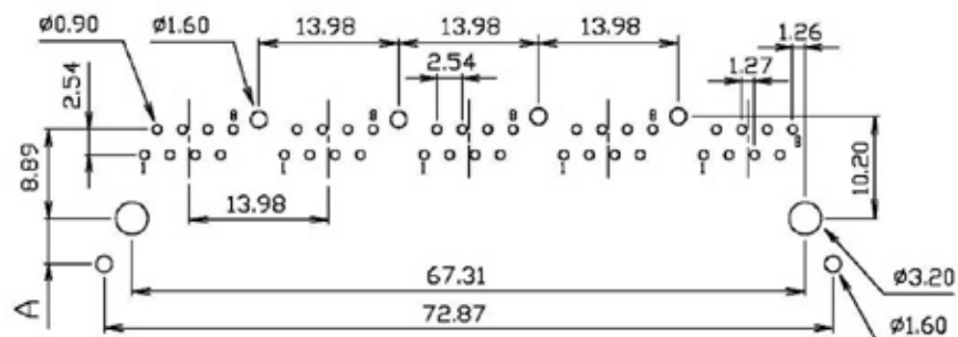
PC Board Layout Ref.
