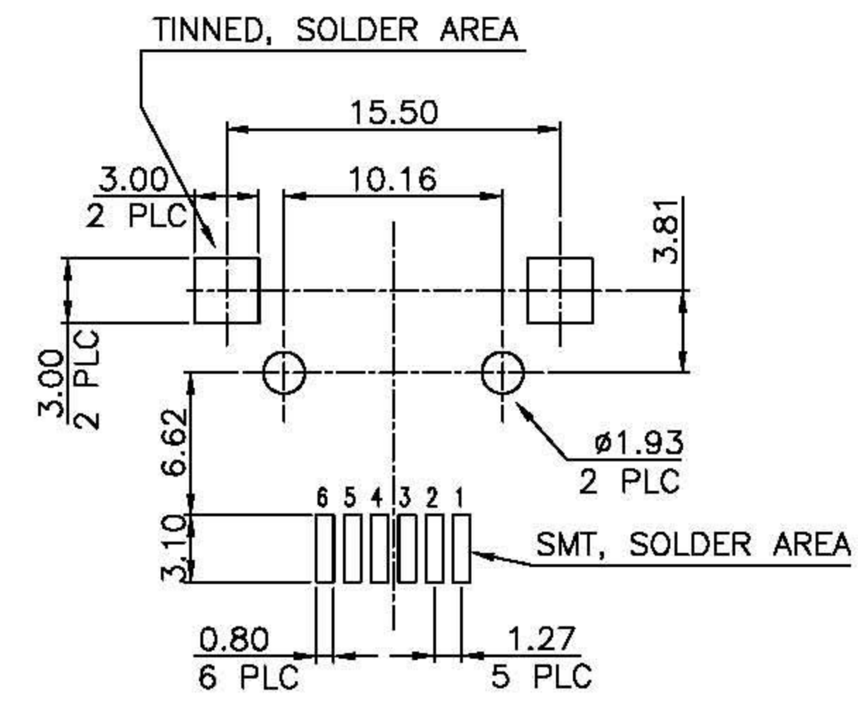
PCB LAYOUT
