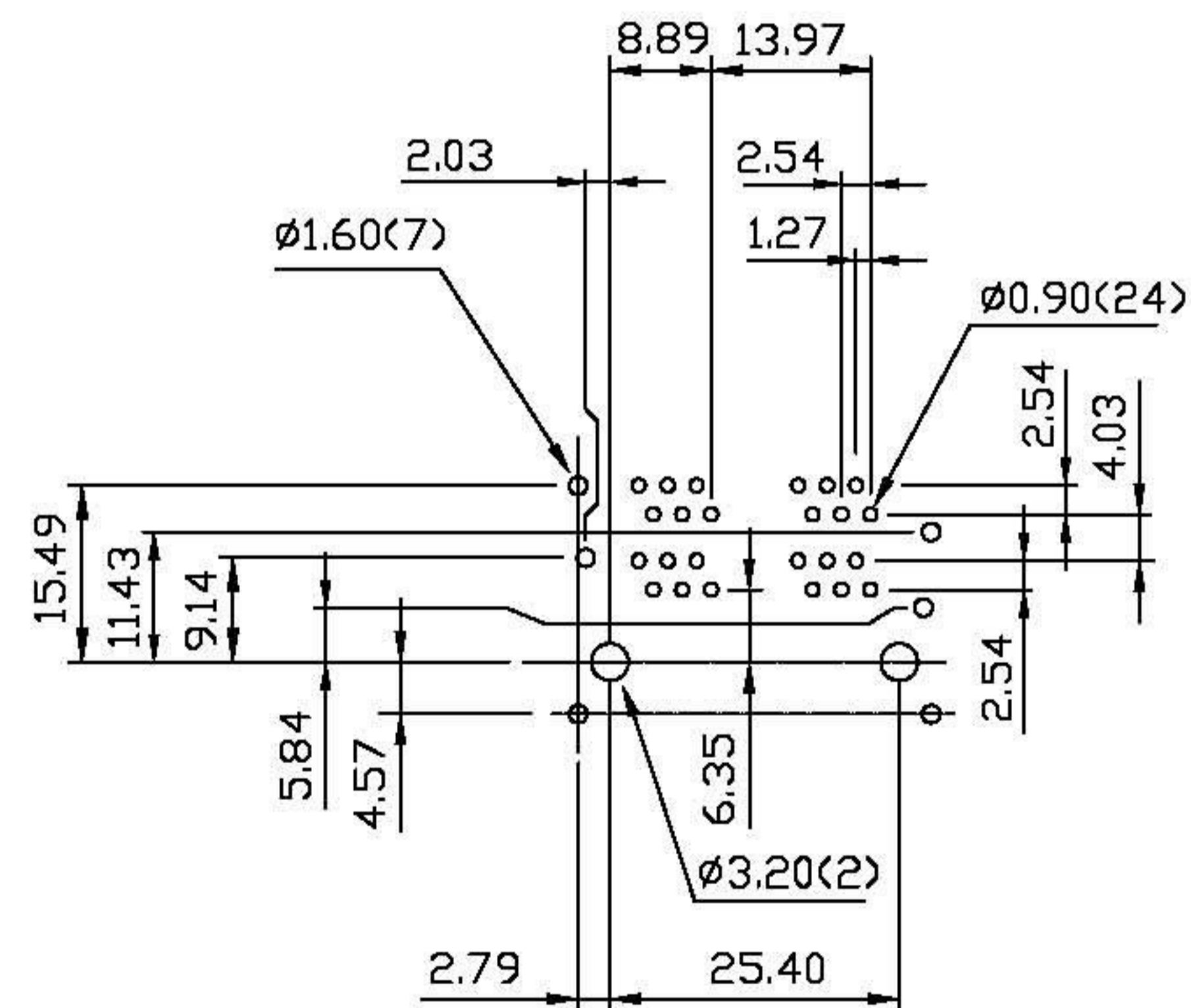
PCB LAYOUT
