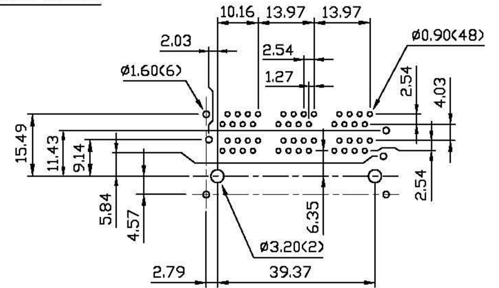
PCB LAYOUT
