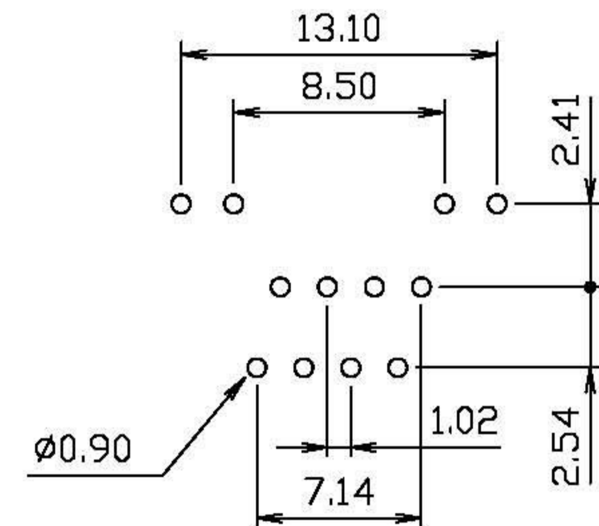
PCB LAYOUT
