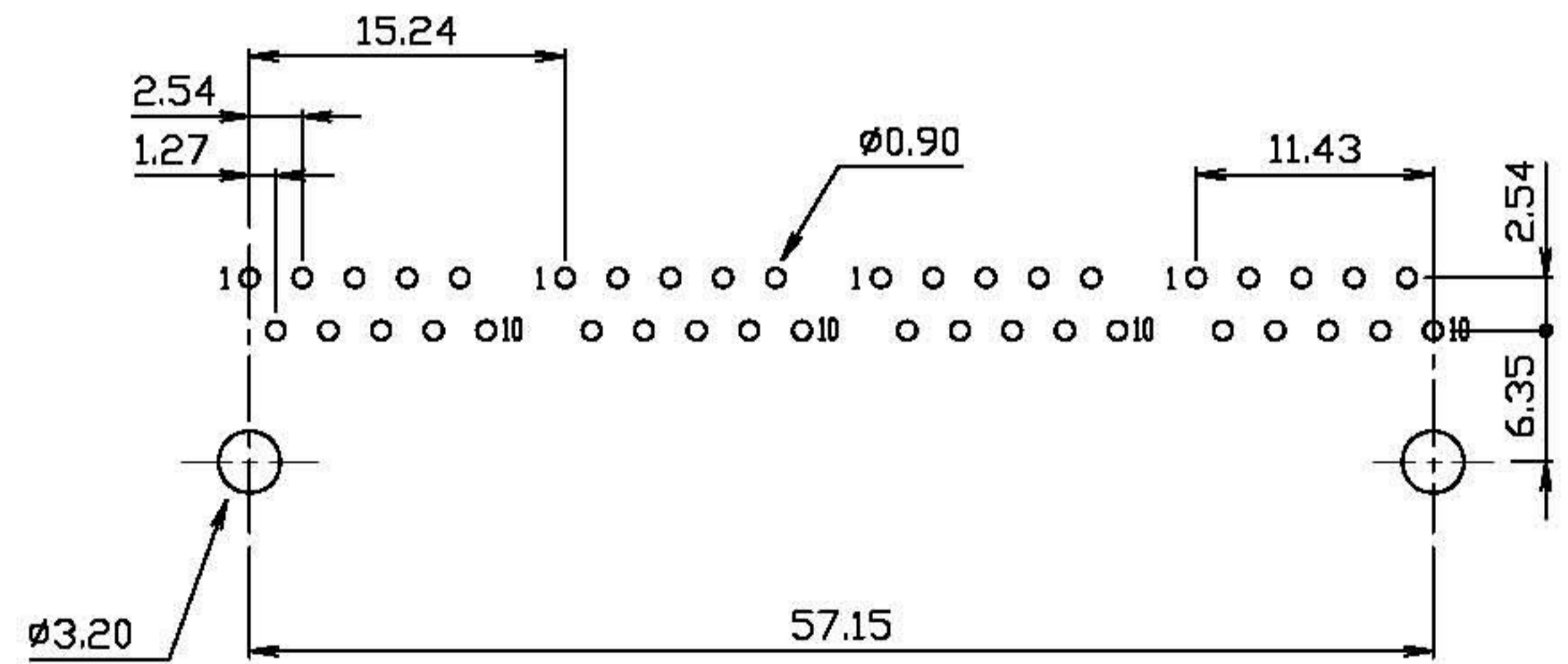
PC Board Layout Ref.
