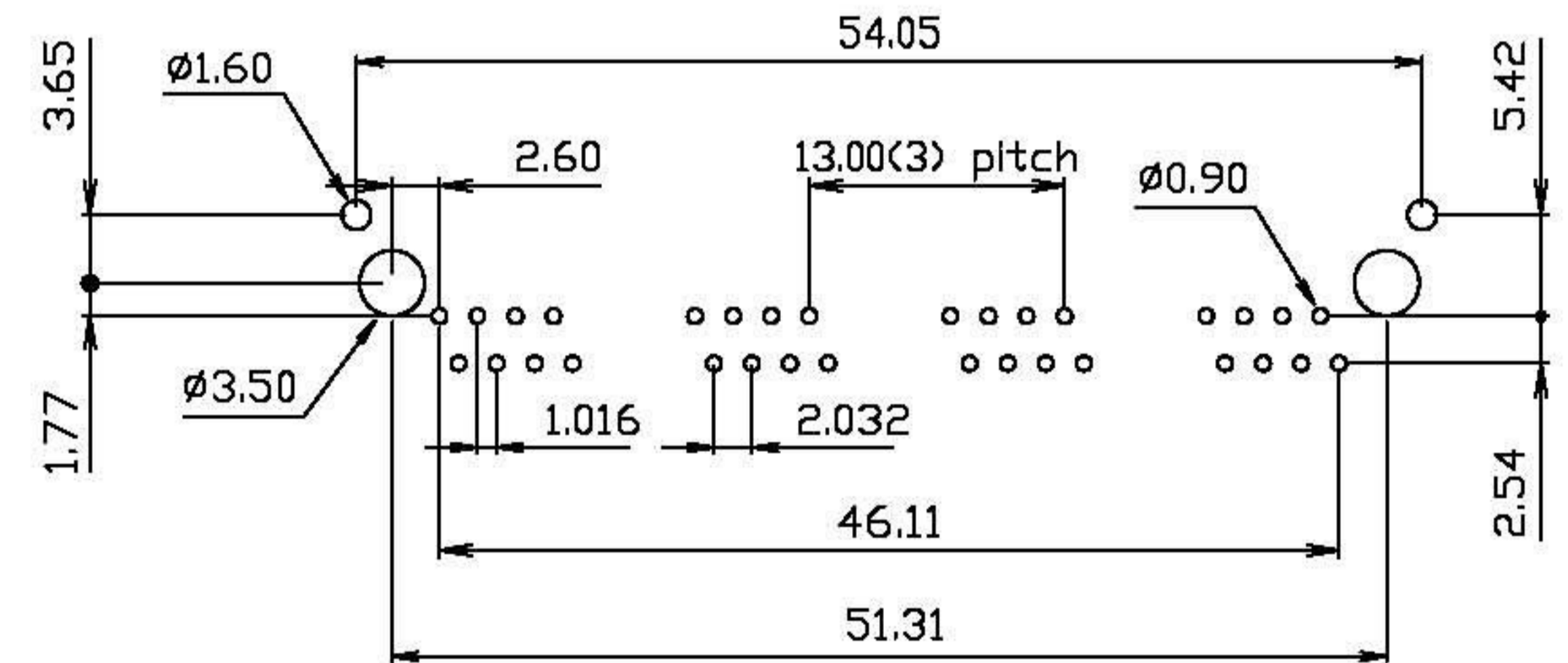
PCB LAYOUT
