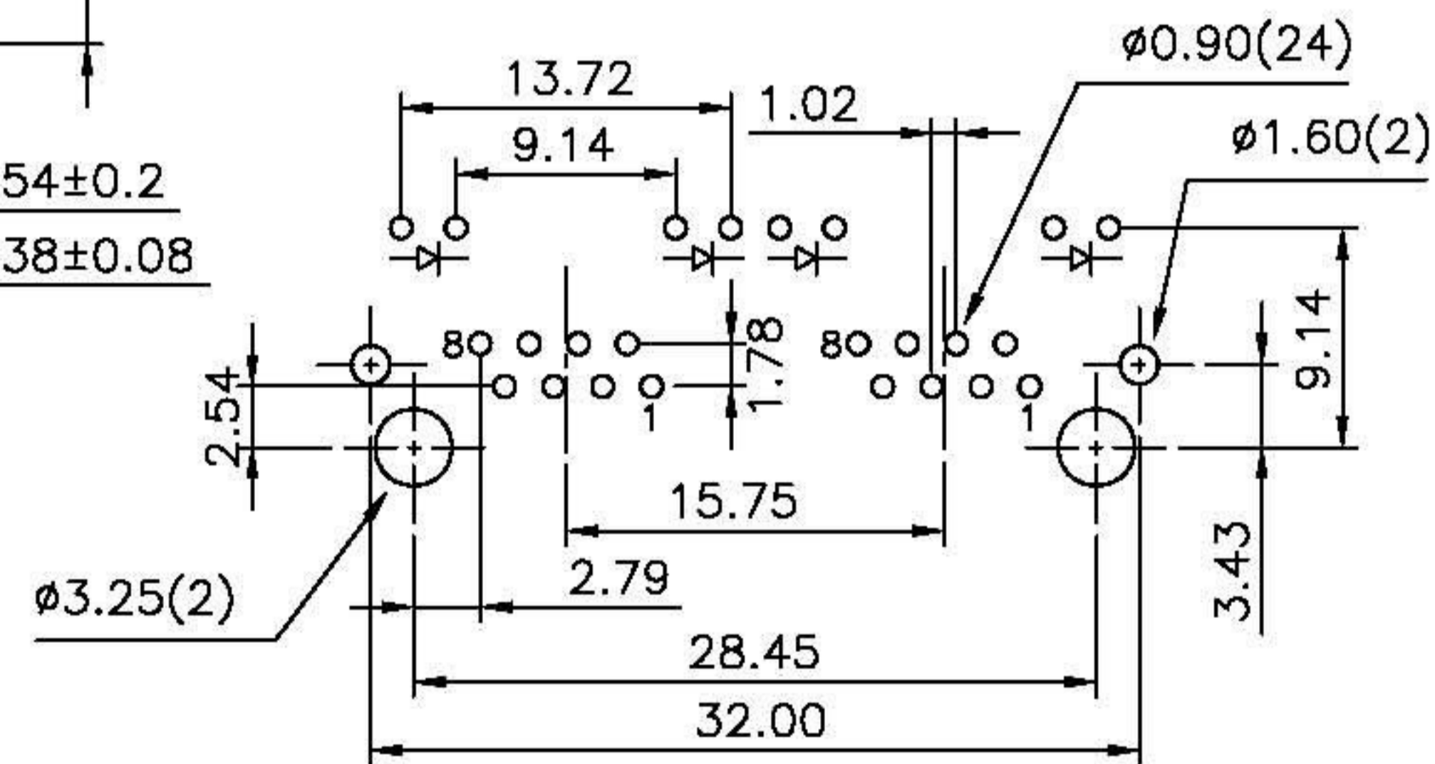
PCB LAYOUT (Ref.)
