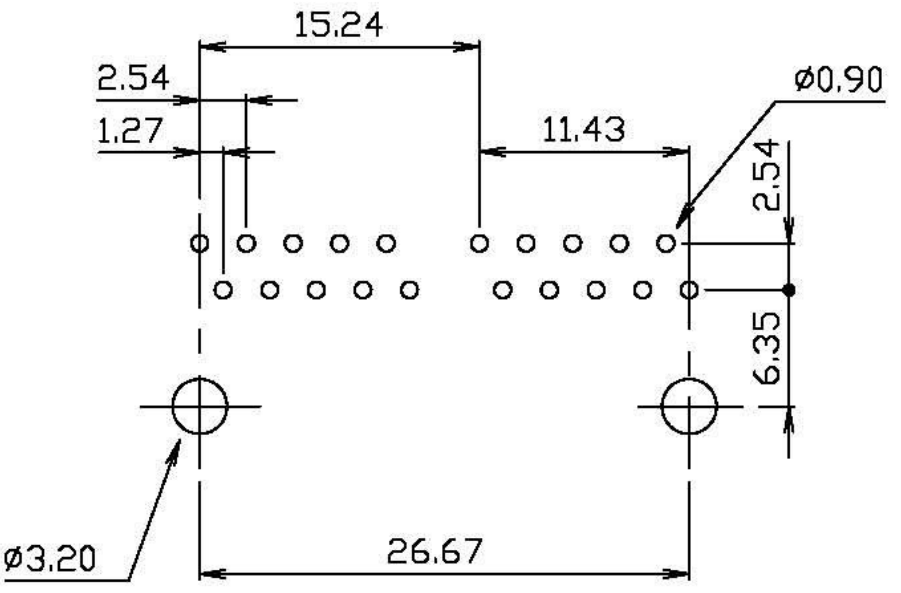
PC Board Layout Ref.
