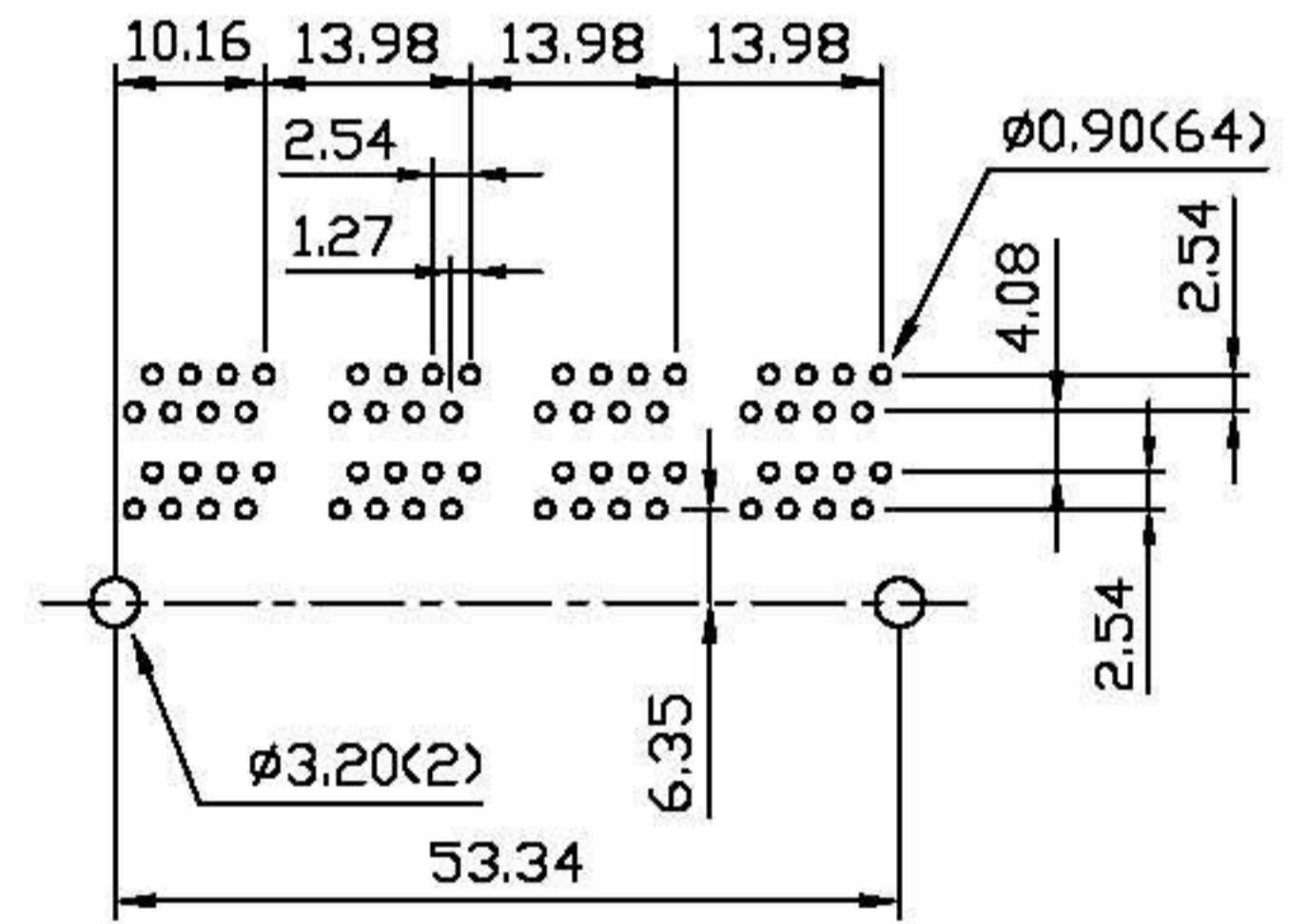
PCB LAYOUT
