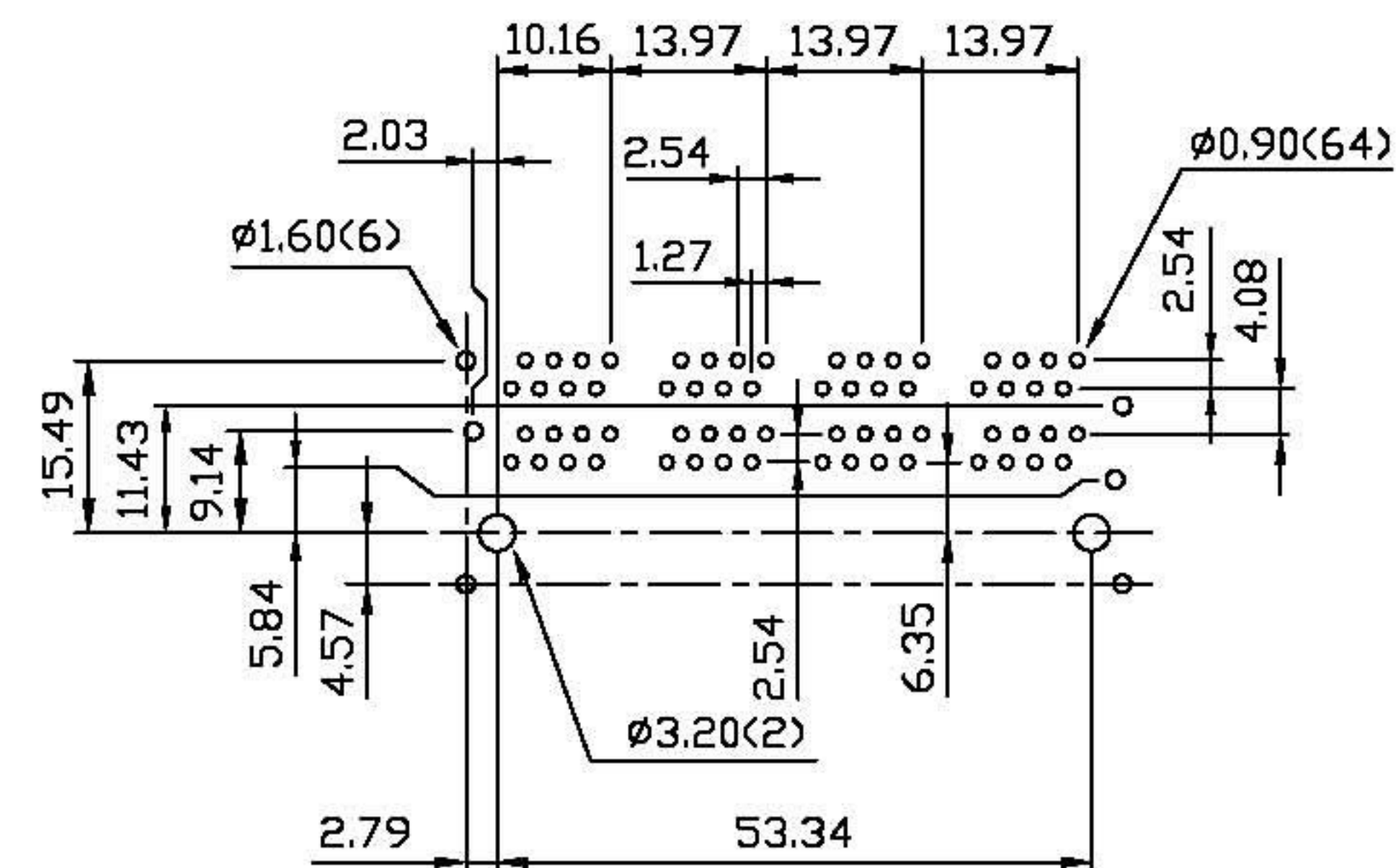
PCB LAYOUT
