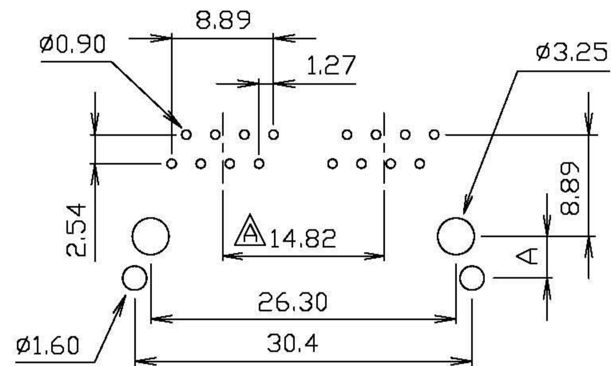
PC Board Layout
