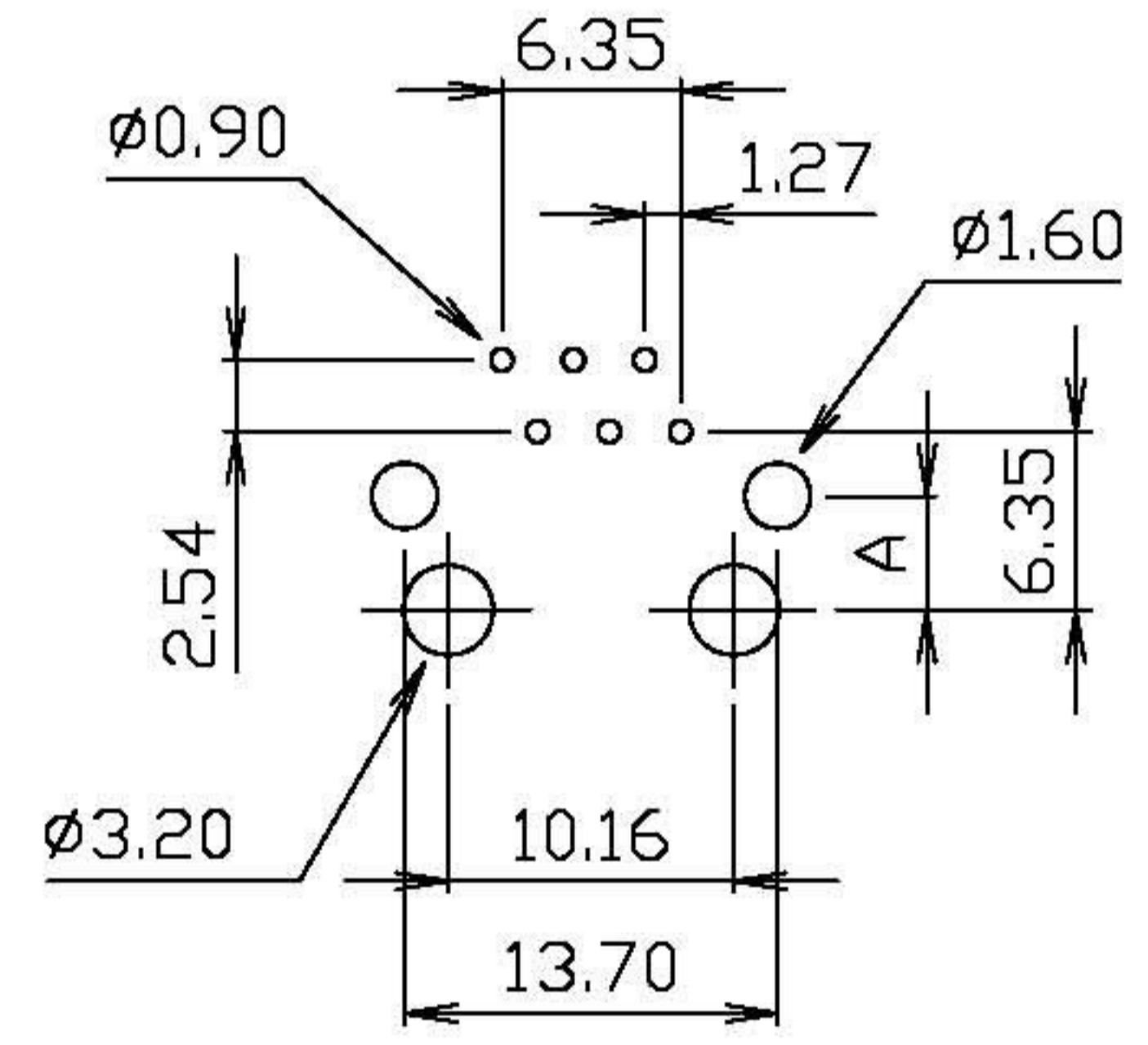
PC Board Layout
