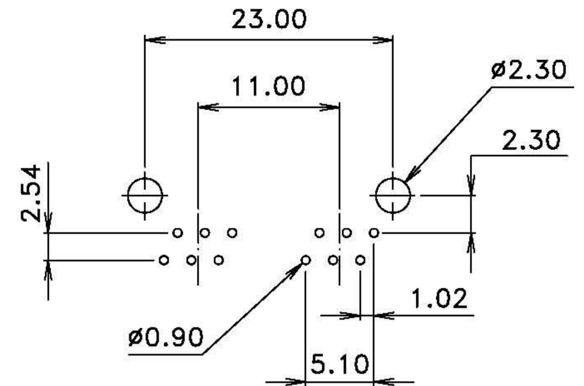
PC Board Layout
