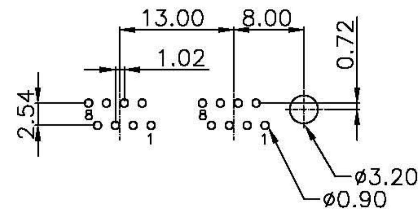
PCB LAYOUT Ref.
