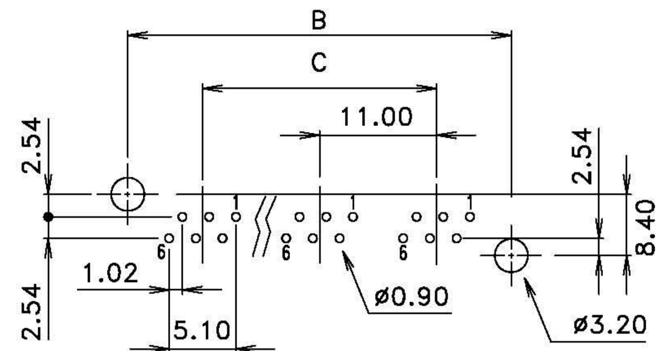
PC Board Layout
