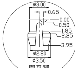
SPLIT-PEGS
