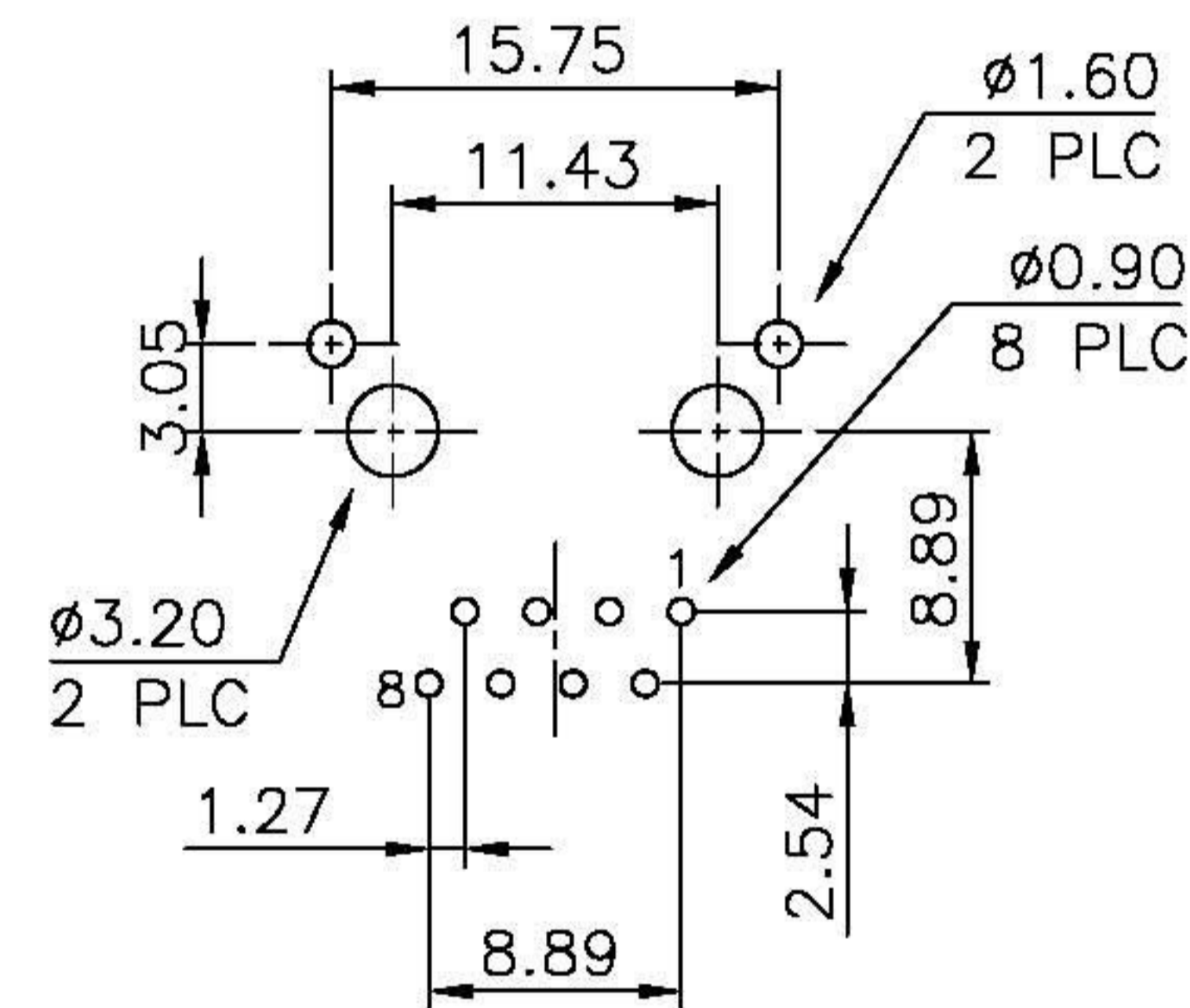
PC Board Layout Ref.
