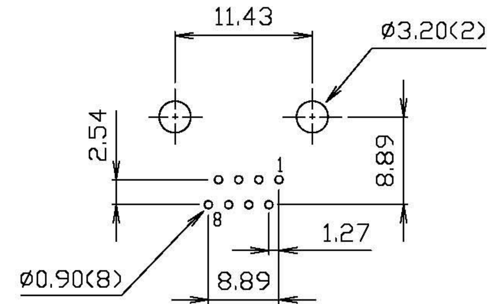
PC Board Layout Ref.
