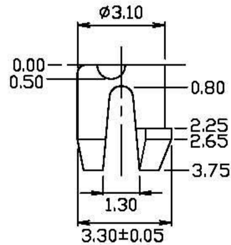
DETAIL X
