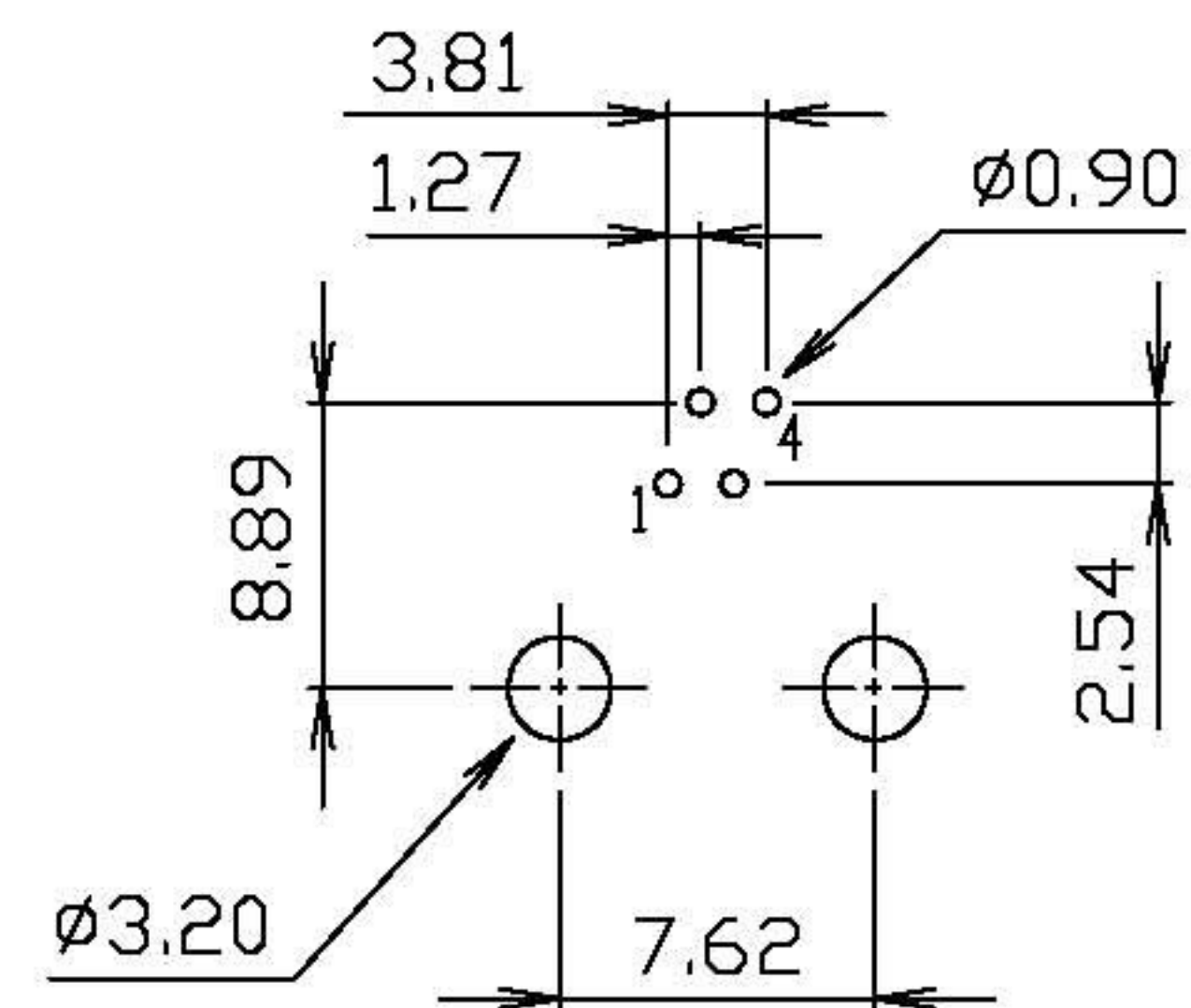
PCB LAYOUT Ref.
