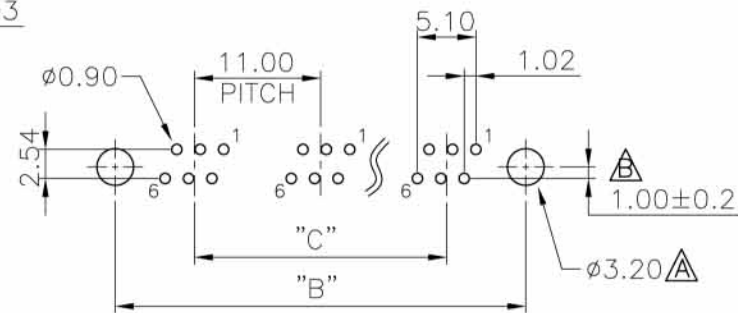
PCB LAYOUT Ref.
