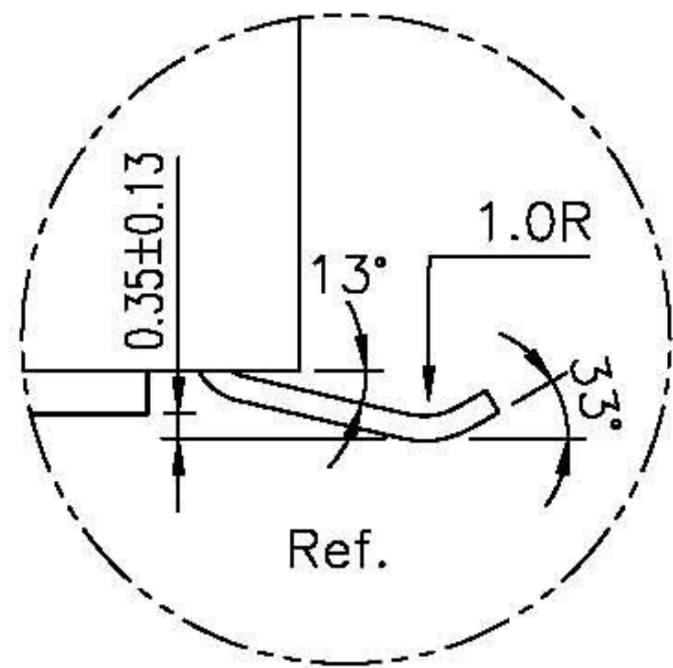
DETAIL X
