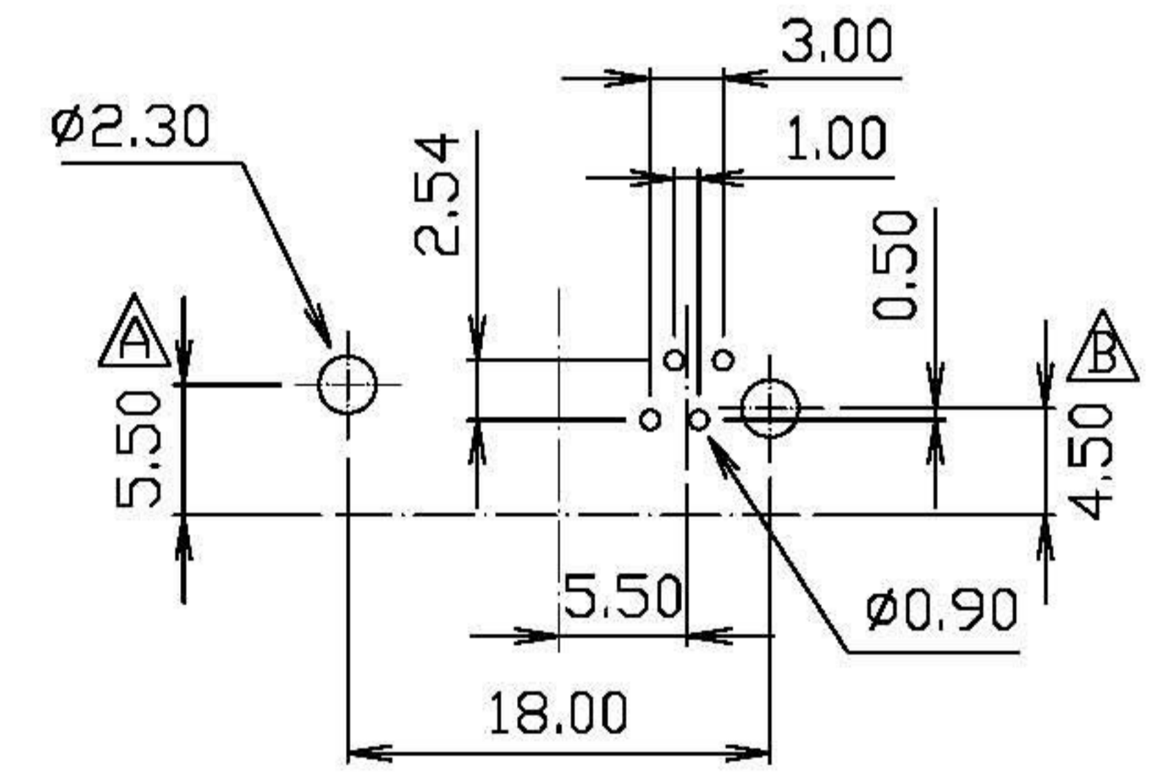
PC Board Layout
