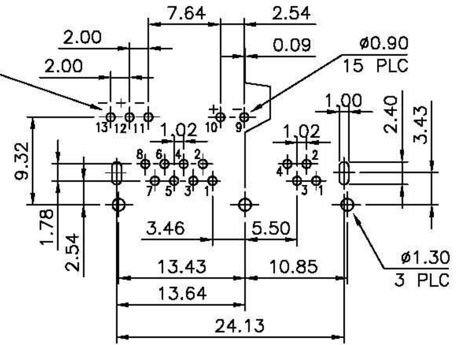
PCB LAYOUT Ref.
