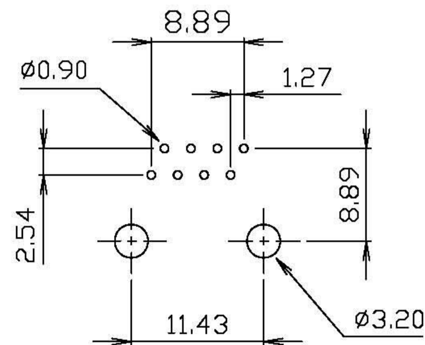
PC Board Layout
