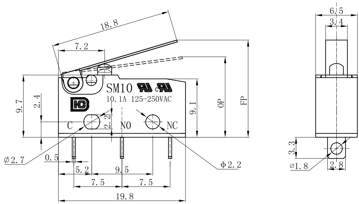
SCHEMATIC
